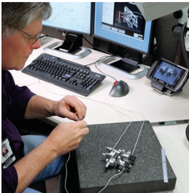
Extensometer Calibration
